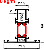
64-6500-6501 1.714 kg/m
