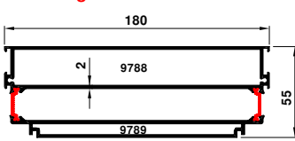
64-9788-9789 4.456 kg/m
