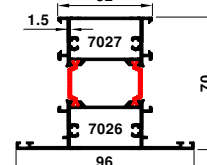
70-7027-7026 1.989 kg/m
