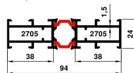
2705-2705 1.485 kg/m
